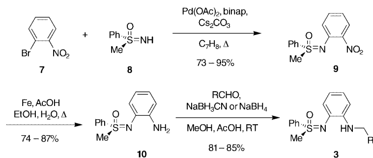
Scheme 2. Synthesis of benzene-bridged aminosulfoximines 3 . Binap = 2,2'-bis(diphenylphosphanyl)-1,1'-binaphthyl.
